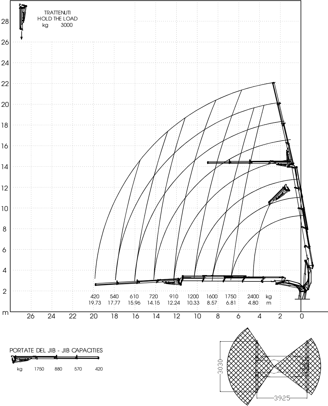
Front Reach-Jib
