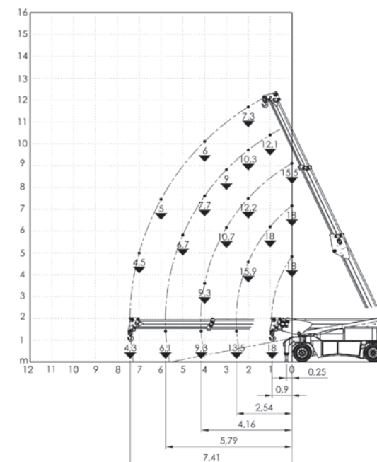
FRONT COMPASS TYPE OUTRIGGERS
