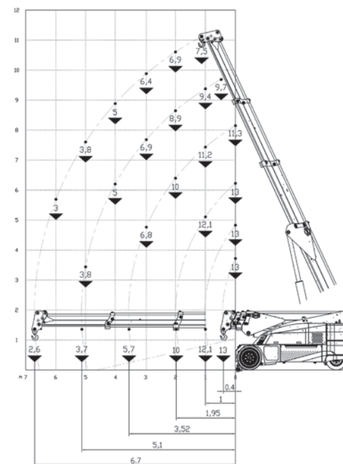
HOOK ON STABILISING BAR
