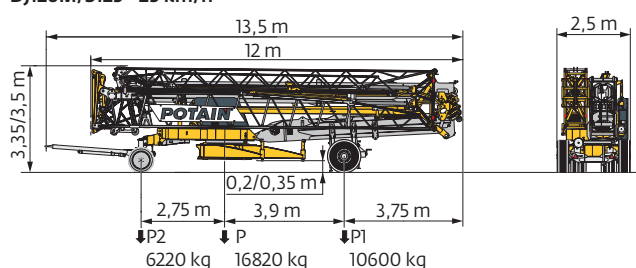
DJ126M/S125 - 25 km/h
